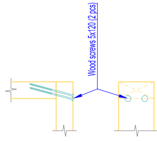
DETAIL "B" / M 1:10@A3
