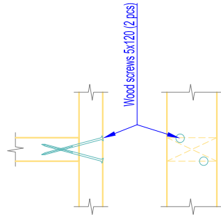
DETAIL "A" / M 1:10@A3
