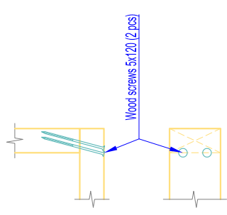
DETAIL "B" / M 1:10@A3
