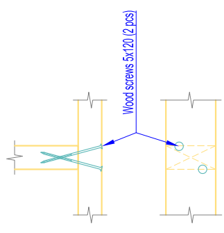
DETAIL "A" / M 1:10@A3
