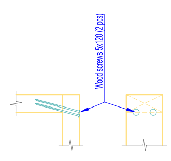
DETAIL "B" / M 1:10@A3
