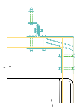
HINGE ASSEMBLY / M 1:10@A3
