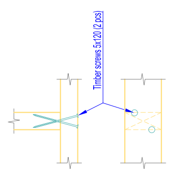
DETAIL "A" / M 1:10@A3
